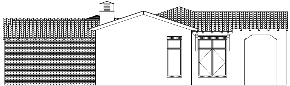
Side Elevation 1
