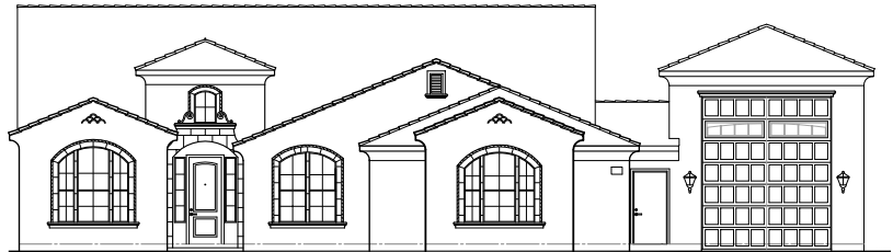
Front Elevation 'D' Opt. RV Garage
