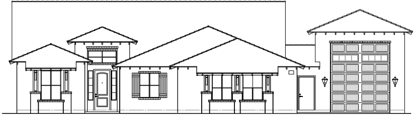
Front Elevation 'B' Opt. RV Garage
